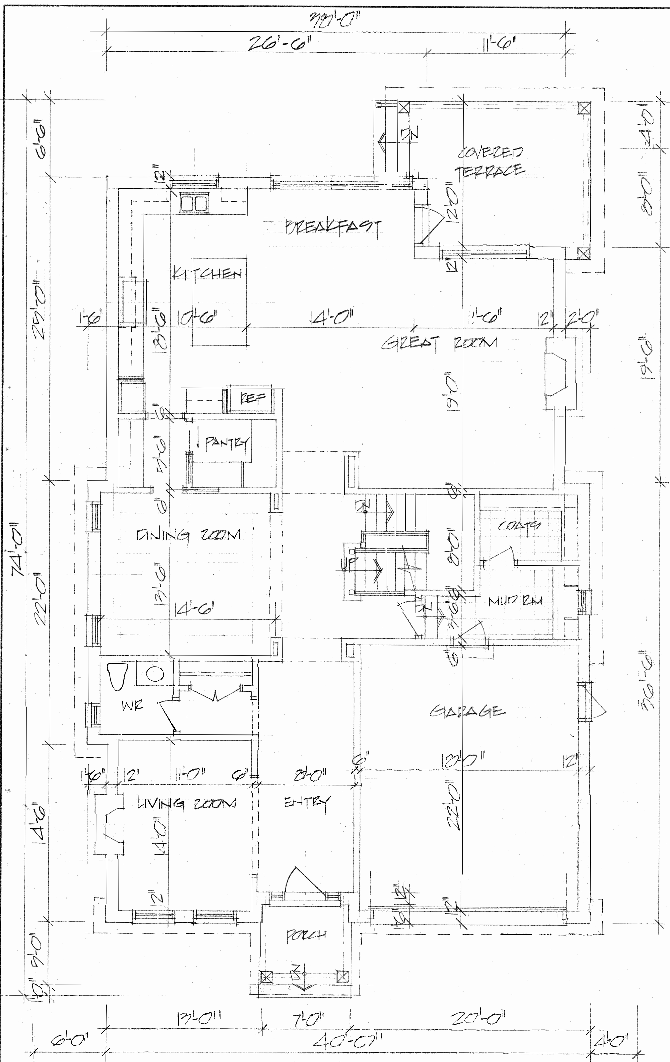
GROUND FLOOR PLAN FLOOR AREA = 1940 SQ FT BUILDING AREA = 2597 "
